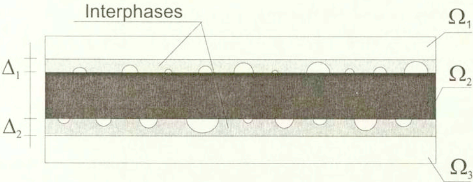
FIG. 5. Interface micro-geometry of stratified composite.
