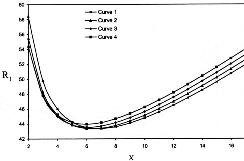
FIG. 5. The variation of Rayleigh number ( R_1 ) with wave number ( x ) for p_1 = 7 , Pe = 4 , T_1 = 20 , P = 4 , \varepsilon = 0.7 , z = 0.25 ; Q_1 = 1 for curve 1, Q_1 = 2 for curve 2, Q_1 = 3 for curve 3 and Q_1 = 4 for curve 4.
